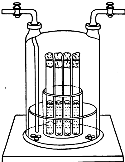
FIG. 137.—Bulloch's jar.
